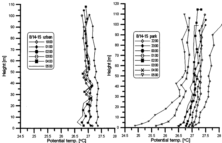
Fig. 2 Potential temperature profile measured by the kytoon systems at points P (park) and U (town).
