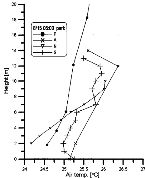
Fig. 3 Air temperature profiles in the park at 05:00 JST. P: above the lawn surface measured by the kytoon system. A, N, and S: below the tree crown in the forest area measured by thermocouples.
