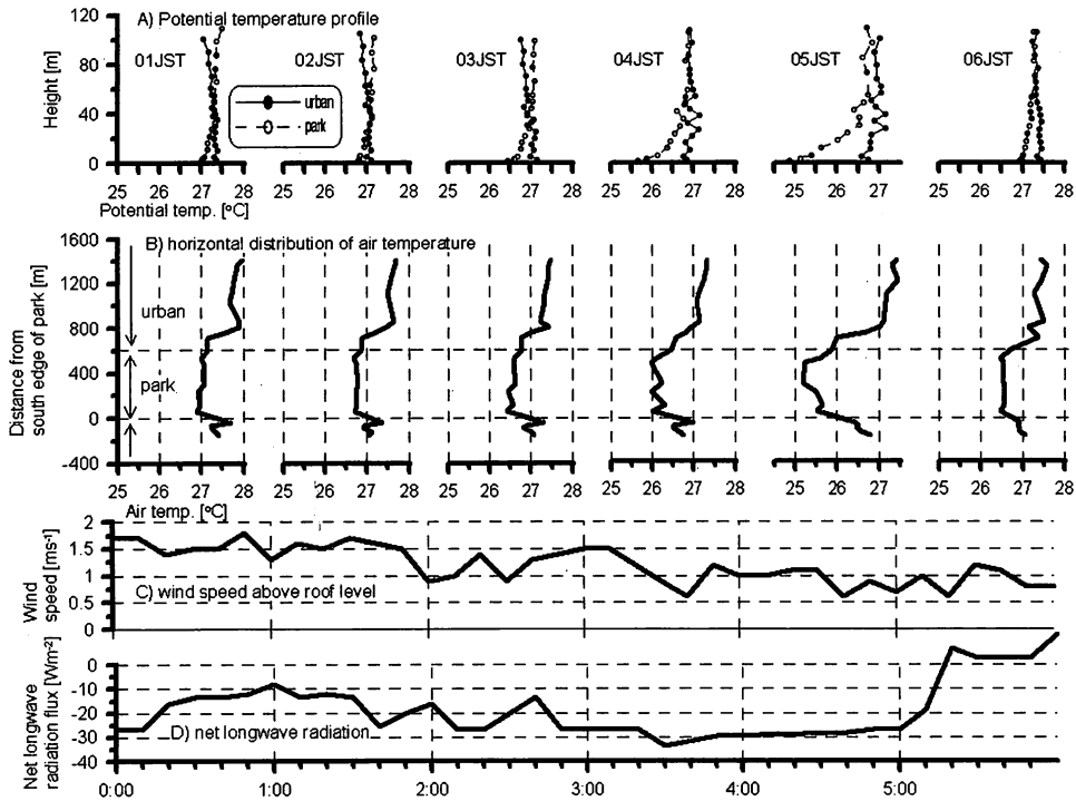
Fig. 5 Time series of potential temperature profiles (A), horizontal distribution of air temperature along the line X-Y in Fig. 1 (B), roof-level wind speed (C), and net longwave radiation flux at a lawn surface in the park (D).
